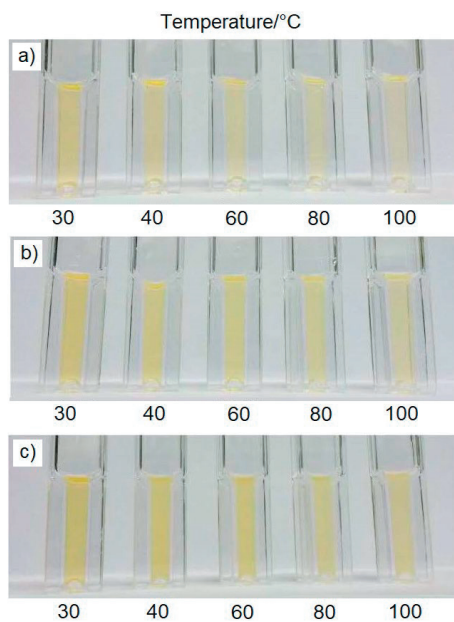
Fig. S1. Stability of lycopene nanodispersion stabilized by: a) soy lecithin, b) sodium caseinate, and c) a mixture of soy lecithin and sodium caseinate in the ratio 1:1, incubated at different temperatures for 1 h
