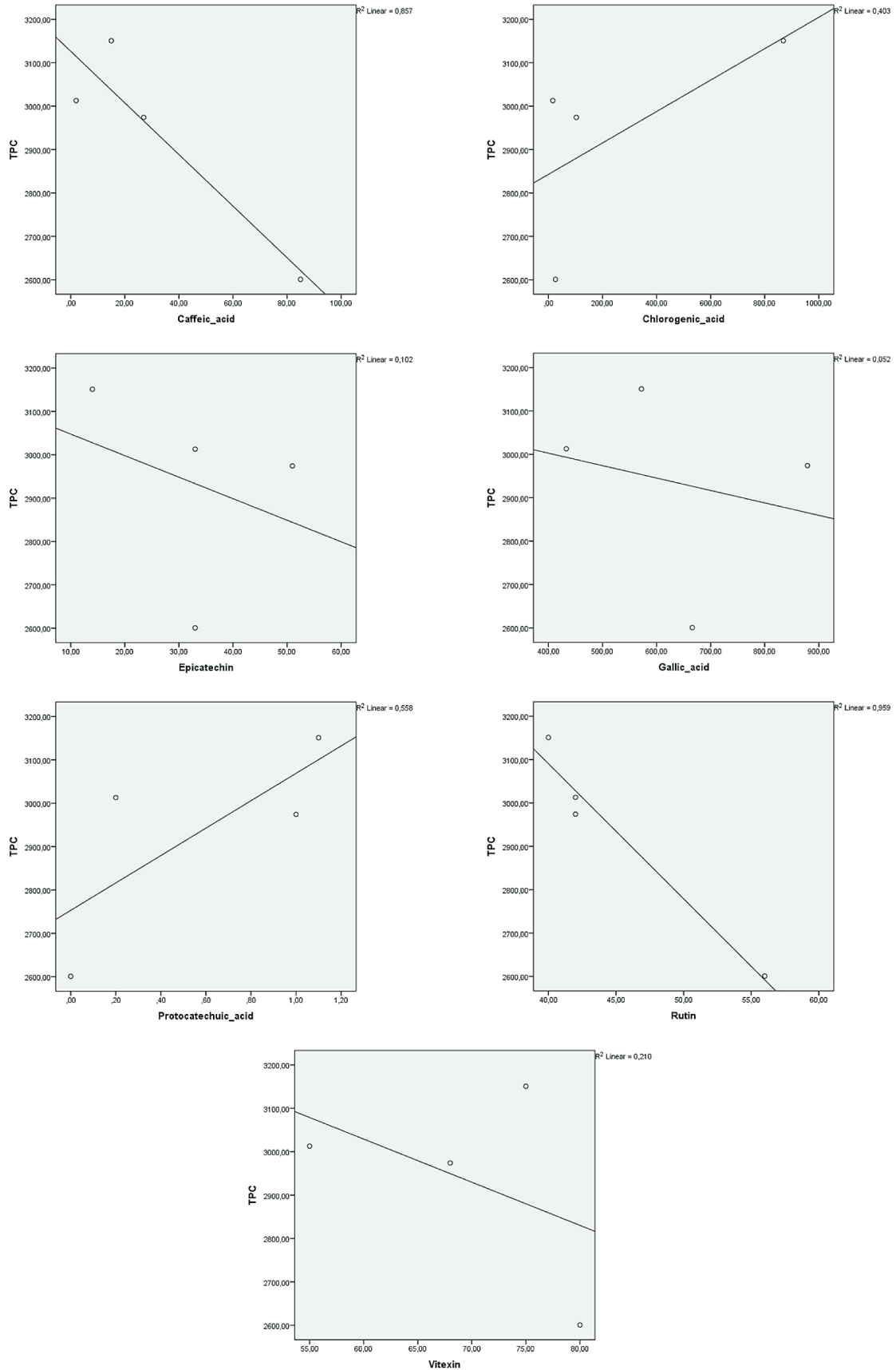
Fig. S2. Spearman's correlation between the identified compounds and the measured total phenolic content (TPC)
