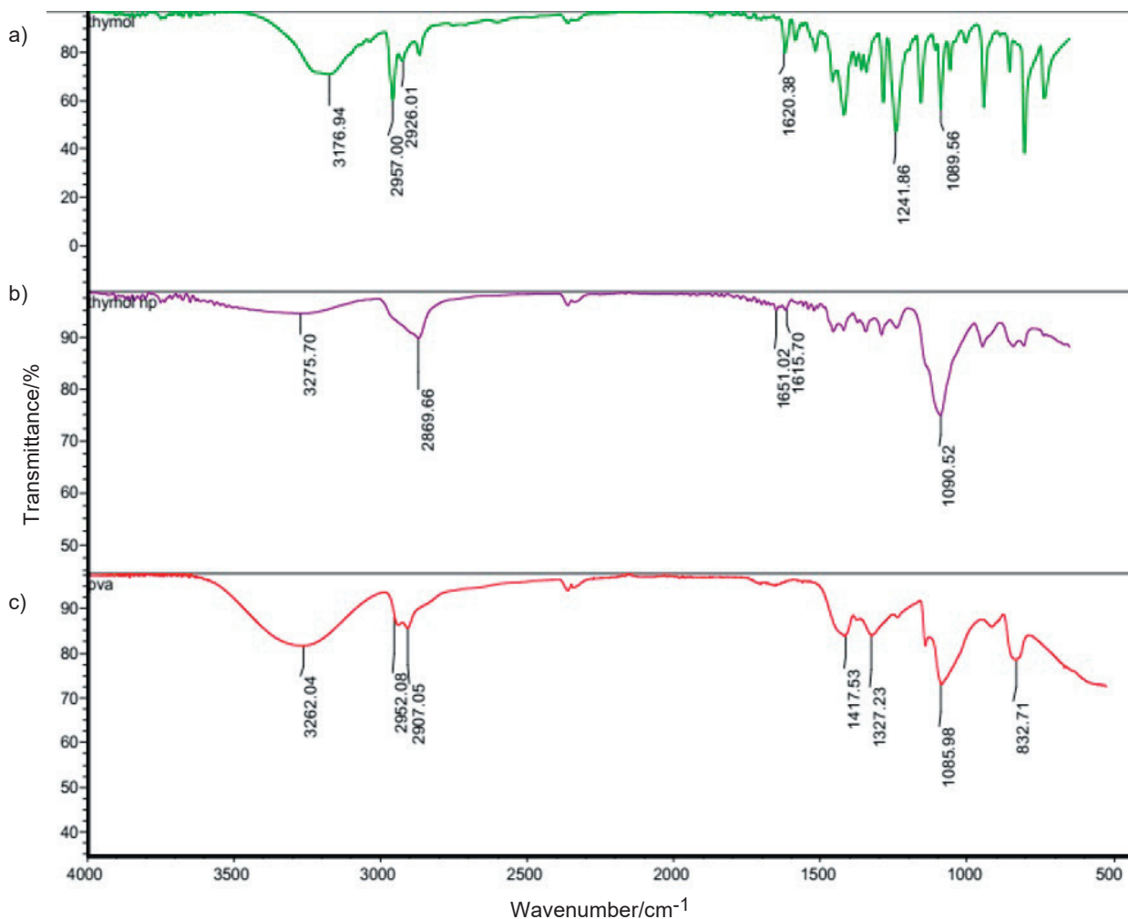
Fig. S1. FTIR spectrum for: a) thymol, b) thymol nanoparticles, and c) polyvinyl alcohol
