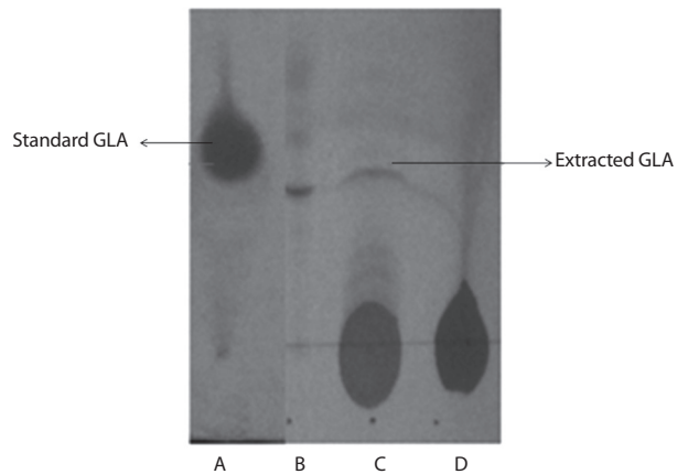
Fig. 3. Comparison of isolated \gamma -linolenic acid (GLA) with standard GLA by thin layer chromatography: A=standard GLA, B=extraction method 3, C=extraction method 1 and D=extraction method 4
